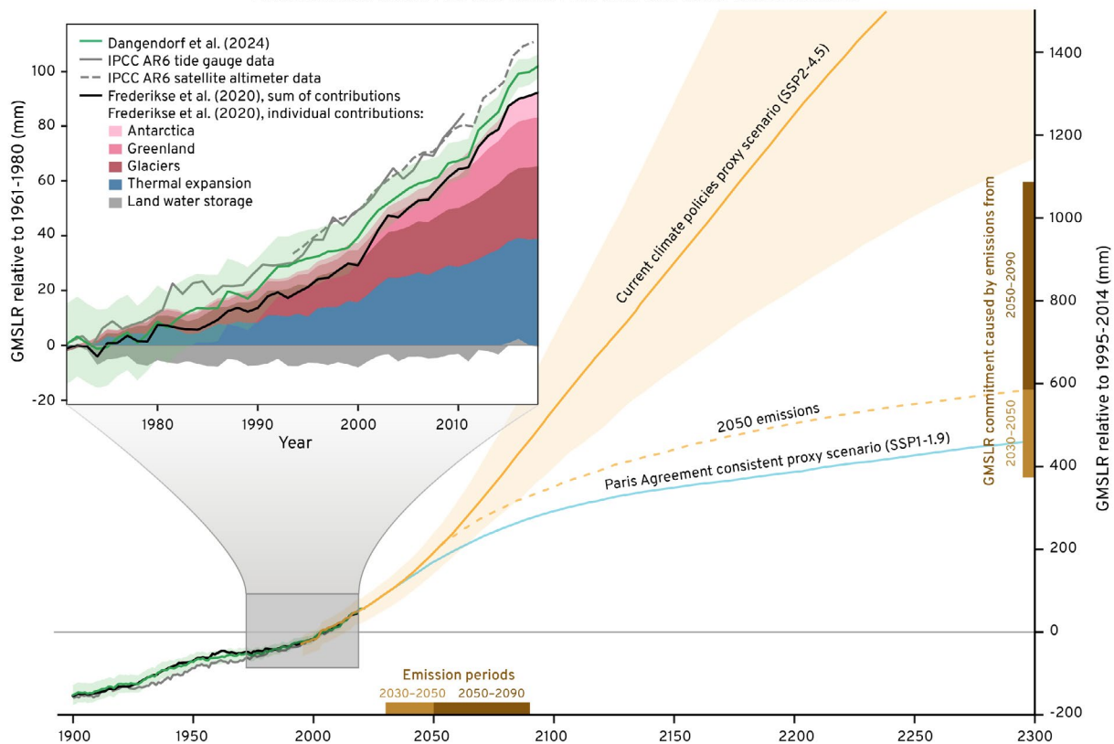
Figure 2. GMSLR and future sea level rise commitments. IPCC Sixth Assessment Report (AR6) historical GMSLR data (dark grey, central estimate) and reconstructions. 10 GMSLR projections 11 under SSP2-4.5 as a current climate policy proxy scenario (solid orange, median and 66% model range) and the locked-in GMSLR commitments from corresponding SSP2-4.5 cumulative greenhouse gas emissions in 2050 (dashed orange, median); and median SSP1-1.9 projection as a proxy for a Paris Agreement-consistent scenario (solid light blue). All data are provided in mm relative to 1995–2014. Brown bars indicate illustrative 2030–2050 and 2050–2090 emission periods and the resulting GMSLR commitments by 2300.
