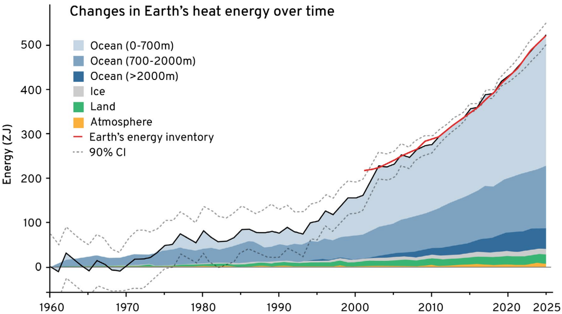
Figure 1. Global energy inventory. OHC annual mean time series from Institute of Atmospheric Physics (Chinese Academy of Sciences) relative to a 1958–1962 baseline, with different ocean layers shown in blue shadings and the grey dashed lines denoting the 90% confidence interval. 7 Also shown are estimates of the land, ice, and atmosphere heat uptake. 8 The Earth's energy inventory (red curve) is derived by first integrating monthly Clouds and the Earth's Radiant Energy System (CERES) EEI data in time to obtain cumulative heat uptake, then converting it to an annual series, and finally aligning the 2005–2025 baseline with that of the summed ocean, land, ice, and atmosphere heat content series. Updated from Cheng et al., 2024. 9
